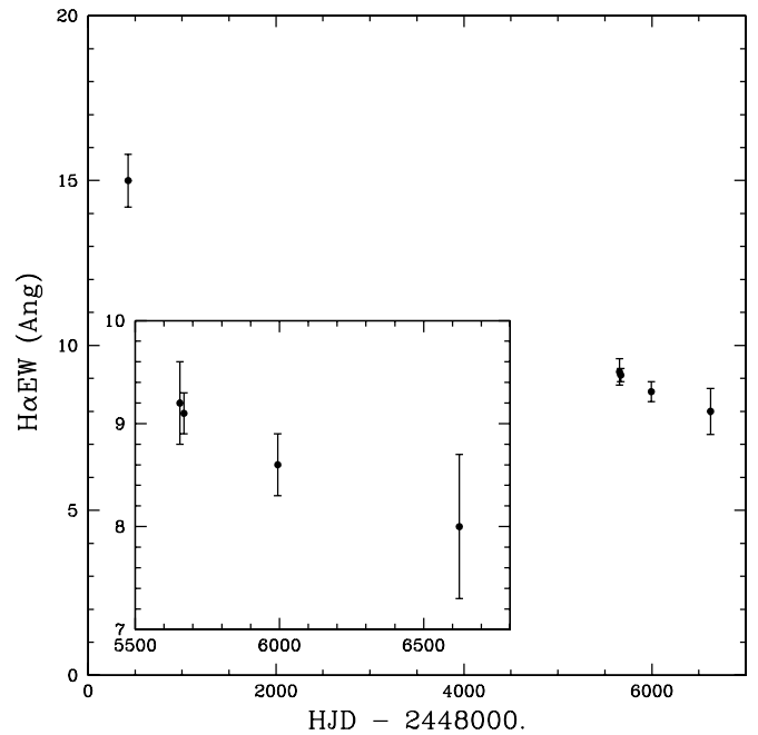
Figure 11. Equivalent width of H\alpha in DK Lac as a function of JD, 1991–2008. The inset shows the most recent data points at sufficient scale to separate a closely spaced pair.
