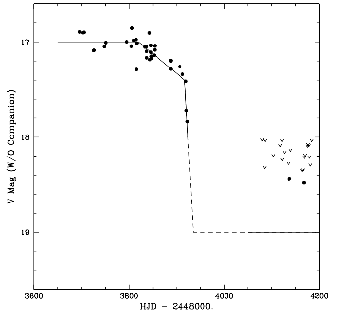
Figure 5. Expanded view of the portion of Figure 1 containing the ingress to the low state. The characterization of the shape of the ingress as two straight lines is adapted from the behavior of high-state/low-state transitions in numerous other VY Scl stars from Honeycutt & Kafka (2004). The level of the low state is fixed at V = 19 using data off the plot to the right (see Figure 1), where the low-state magnitude varies between 18.5 and 19.5. The occasional RoboScope detections in near 18.5 in the plot are presumably the peaks of this distribution of low-state magnitudes.
