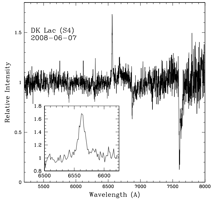
Figure 10. Like Figure 7 except average of four high-state exposures of DK Lac 2008 June 07 (UT) with the KPNO 2.1 m telescope (spectrum S4 as labeled in Figure 2 and Table 3).
