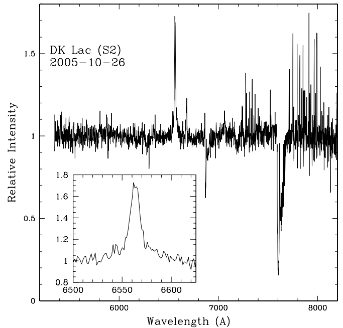
Figure 8. Like Figure 7 except average of three high-state exposures of DK Lac 2005 October 26 (UT) with the WIYN 3.5 m telescope (spectrum S2 as labeled in Figure 2 and Table 3).
