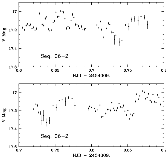
Figure 4. Example of a high-state photometric sequence. The sequence notation refers to labels in Figure 1 and Table 1. Note that the data in these two panels overlap somewhat. The V magnitudes have been corrected for the contribution of the close companion. This plot is for a sequence obtained 2006 October 01 (UT).
