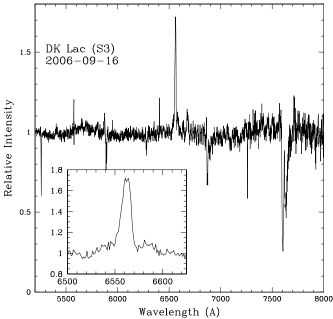
Figure 9. Like Figure 7 except average of two high-state exposures of DK Lac 2006 September 16 (UT) with the MMT telescope (spectrum S3 as labeled in Figure 2 and Table 3).
