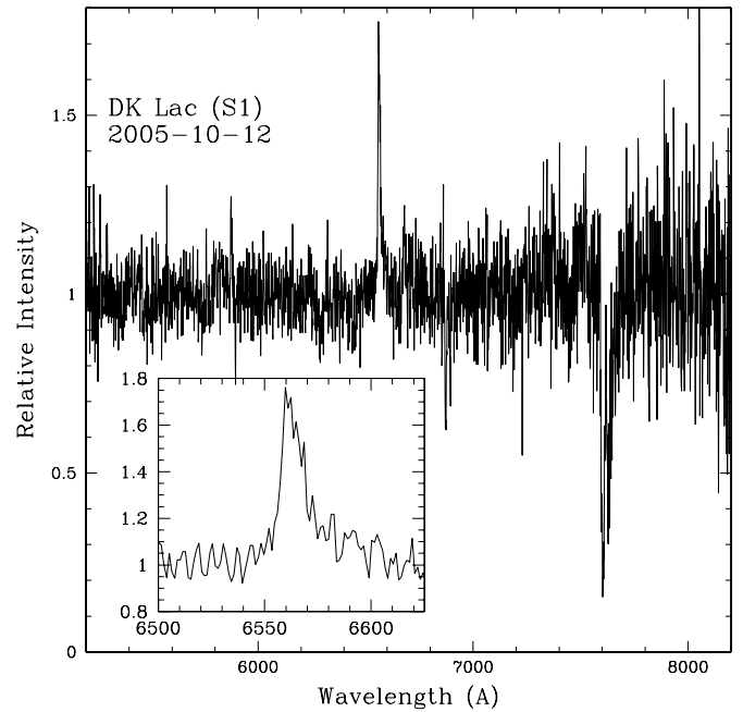
Figure 7. Average of two exposures of DK Lac obtained 2005 October 12 (UT) with the KPNO 2.1 m telescope (spectrum S1 as labeled in Figure 2 and Table 3). The continuum has been normalized to unity and the H\alpha line profile is shown on an expanded scale. No corrections for atmospheric extinction have been applied; therefore the telluric absorption bands remain.
