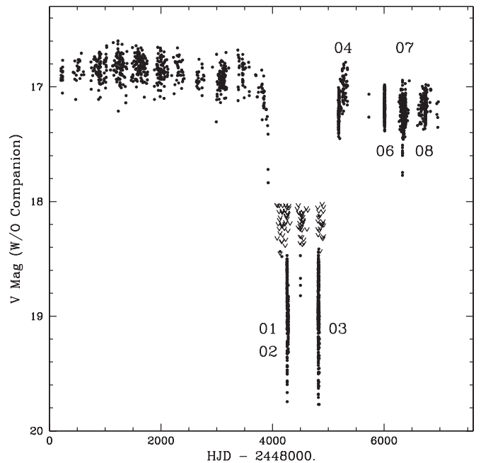
Figure 1. Full light curve of DK Lac from 1990 November 12 to 2009 May 21. The contribution of the companion star has been removed (see the text for details). Error bars have been omitted for clarity. The upper limit symbols during the 2001–2003 low state are from RoboS. The vertical clusters of unresolved points labeled 01 through 08 are continuous sequences of exposures, typically obtained on several successive or nearly successive nights. The sequence root number is the last two digits of the year. A serial number is appended to the sequence root to form the sequence number column in Table 1, and this notation is preserved for plots of the individual sequences (Figures 3 and 4).
