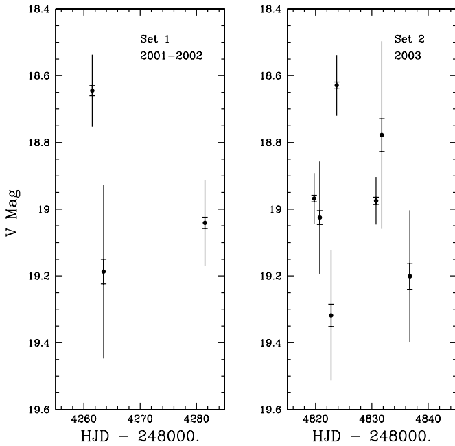
Figure 6. Mean magnitude of the low-state sequences for Set 1 (left) and for Set 2. Sets 1 and 2 each encompass \sim 3 weeks, separated by 1.5 years. The short error bars are for sdm and the longer ones for sds.
