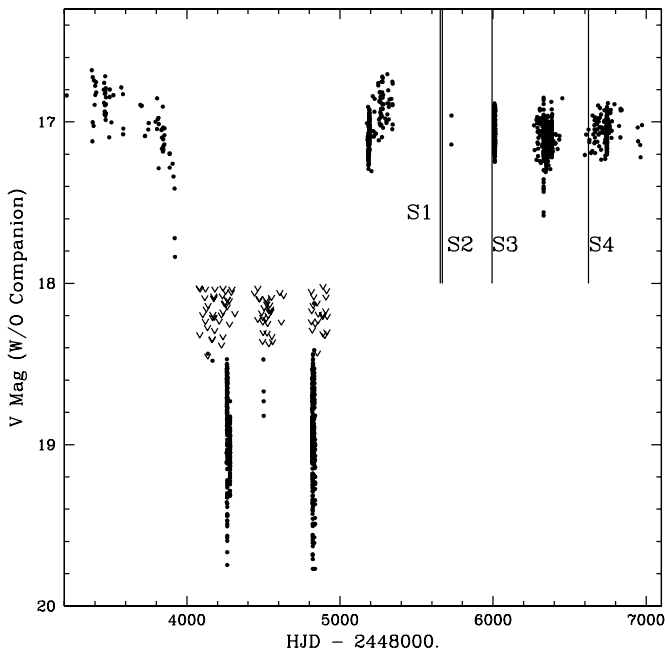
Figure 2. Latter portion of Figure 1 with the times of spectroscopic data marked. The labels for the times of spectral exposures correspond to Column 1 of Table 3.
